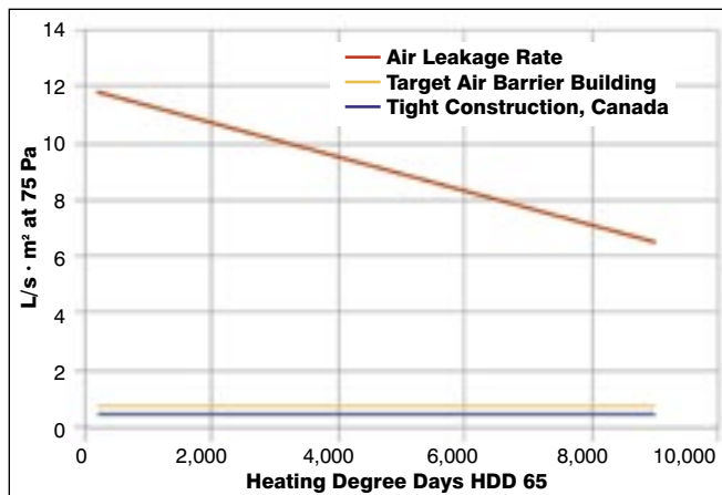
Figure 1: Buildings in the North are tighter than buildings in the South; all are leaky.
